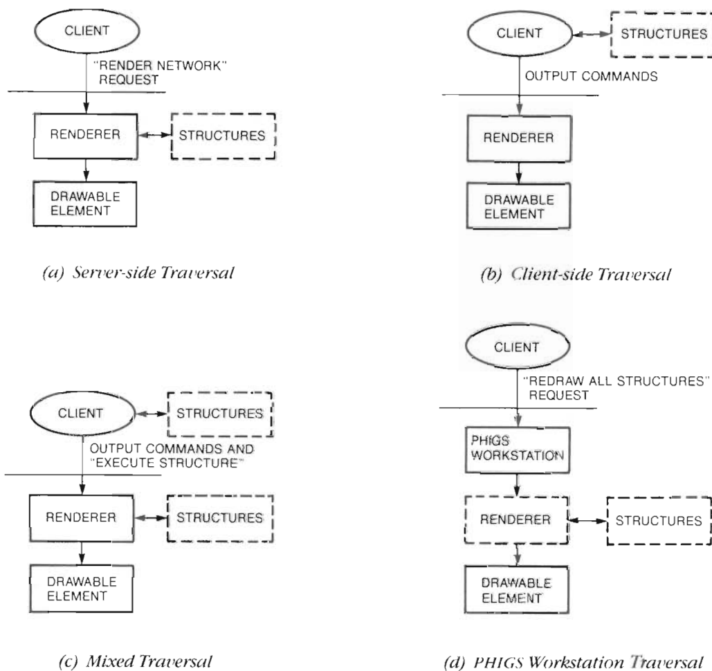
Figure 5 Display List Traversal Options
