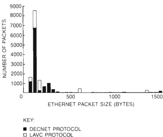
Figure 2 Ethernet Packet Size Distribution for Local Paging
