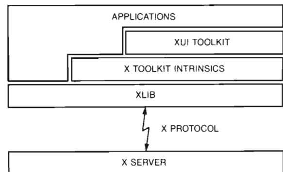
Figure 1 DECwindows Architecture
