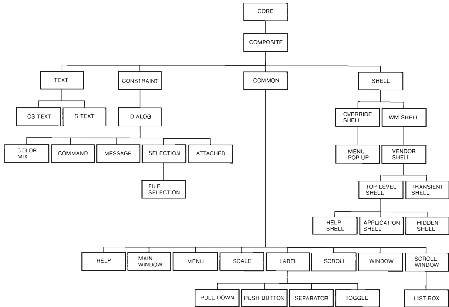
Figure 2 XUI Toolkit Widget Class Hierarchy
