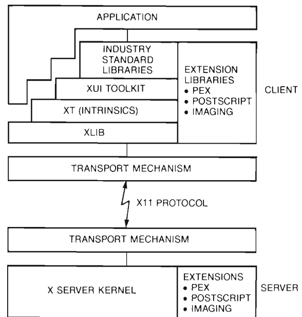
Figure 2 DECwindows Architecture
