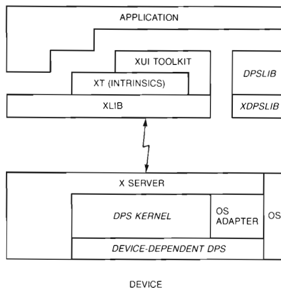
Figure 2 The Extension and the Display PostScript System
