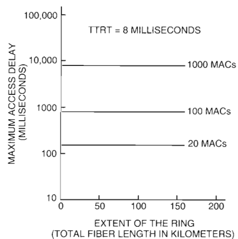
Figure 7 Maximum Access Delay as a Function of the Extent of the Ring
