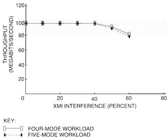
Figure 4 Receive Throughput as a Function of XMI Interference for an XMI (CPU) Bus Configuration
