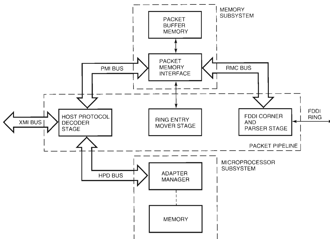
Figure 2 DEMFA Block Diagram
