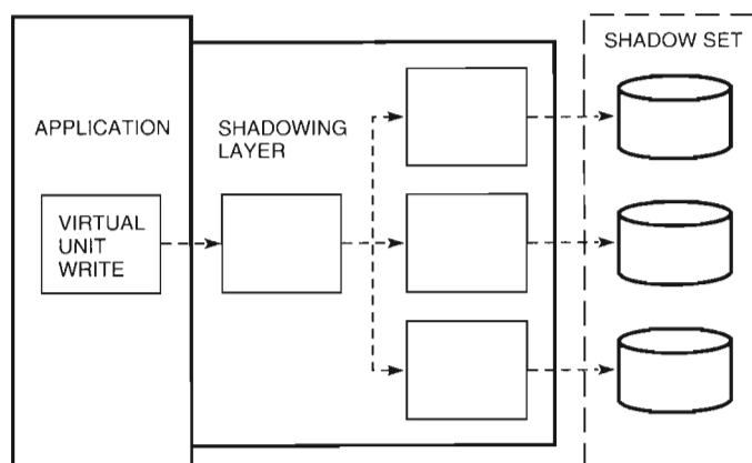
Figure 4 Shadow Set Write Operation
