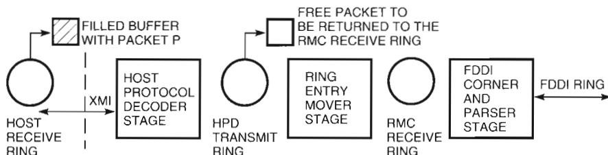
(d) Receive Stream - Packet in the Host Memory on the Host Receive Ring
