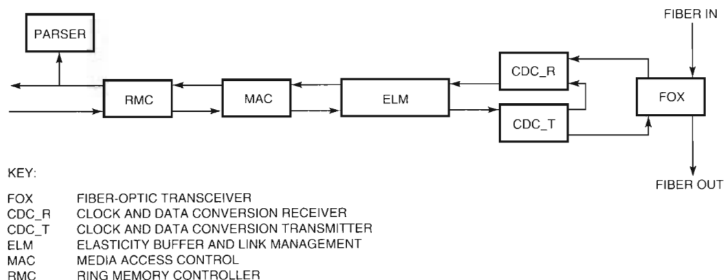
Figure 5 FDDI Corner and Parser Stage
