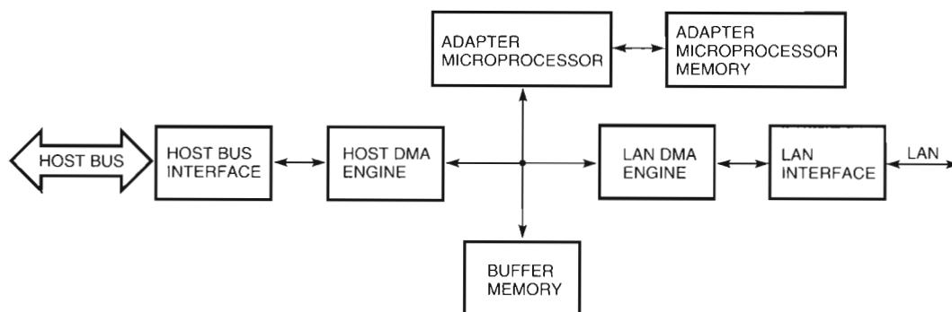
Figure 1 Block Diagram of a Traditional Adapter
