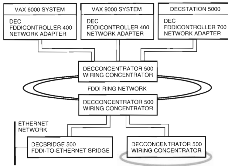
Figure 1 Typical Network Configuration
