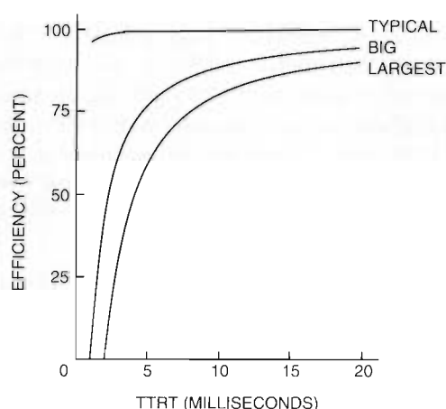
Figure 3 Efficiency as a Function of the TTRT
