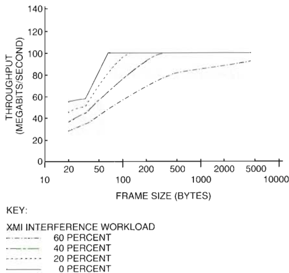
Figure 5 Receive Throughput as a Function of the Frame Size for an XMI (CPU) Bus Configuration
