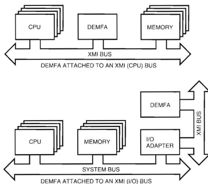
Figure 2 System Types That Support the DEMFA
