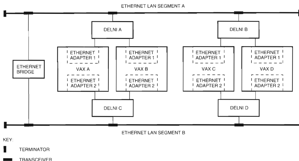
Figure 2 Multiple-adaptor Channel Failure
