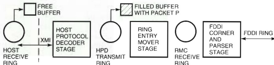
(c) Receive Stream - Packet at the HPD Transmit Ring
