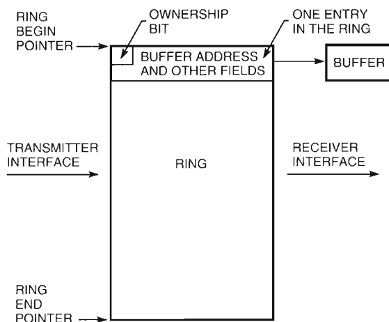
Figure 3 Ring and Ring Interfaces
