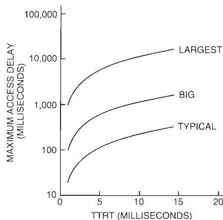
Figure 4 Maximum Access Delay as a Function of the TTRT
