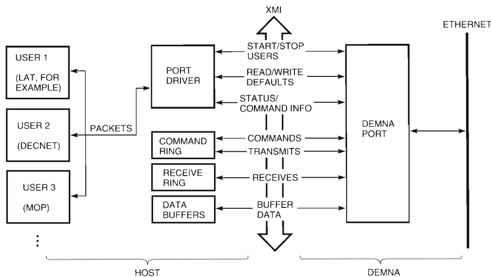
Figure 2 DEMNA Port Interface
