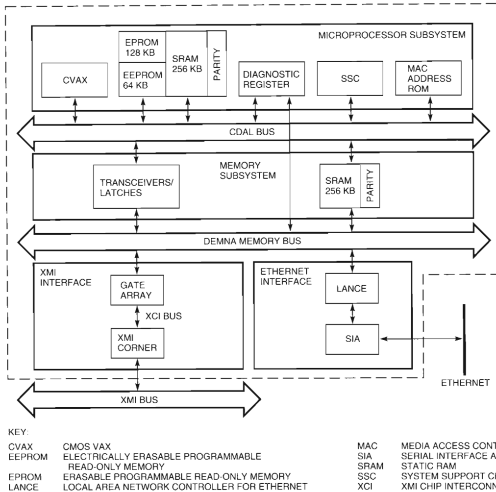
Figure 1 DEMNA Block Diagram
