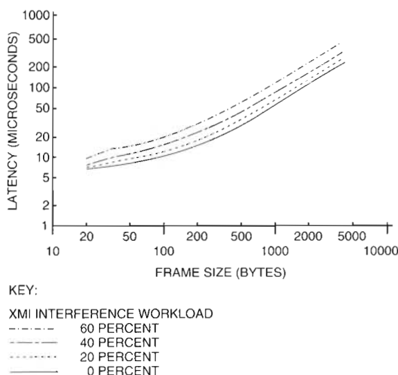
Figure 10 Transmit Latency as a Function of the Frame Size for an XMI (CPU) Bus Configuration
