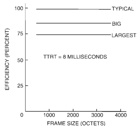
Figure 10 Efficiency as a Function of the Frame Size
