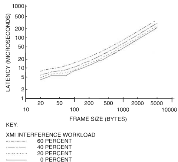
Figure 9 Receive Latency as a Function of the Frame Size for an XMI (CPU) Bus Configuration
