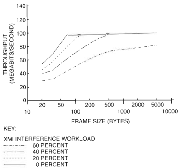
Figure 7 Transmit Throughput as a Function of the Frame Size for an XMI (CPU) Bus Configuration
