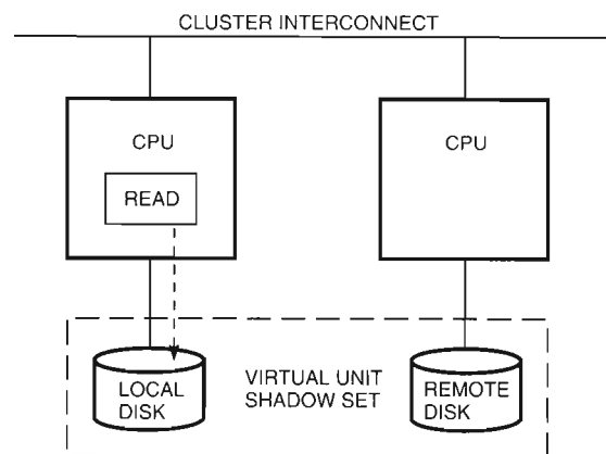
Figure 3 Shadow Set Read Operation
