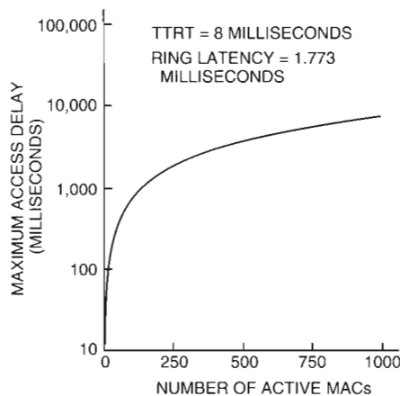
Figure 9 Maximum Access Delay as a Function of the Number of Active MACs
