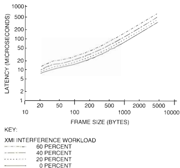
Figure 11 Transmit Latency as a Function of the Frame Size for an XMI (I/O) Bus Configuration
