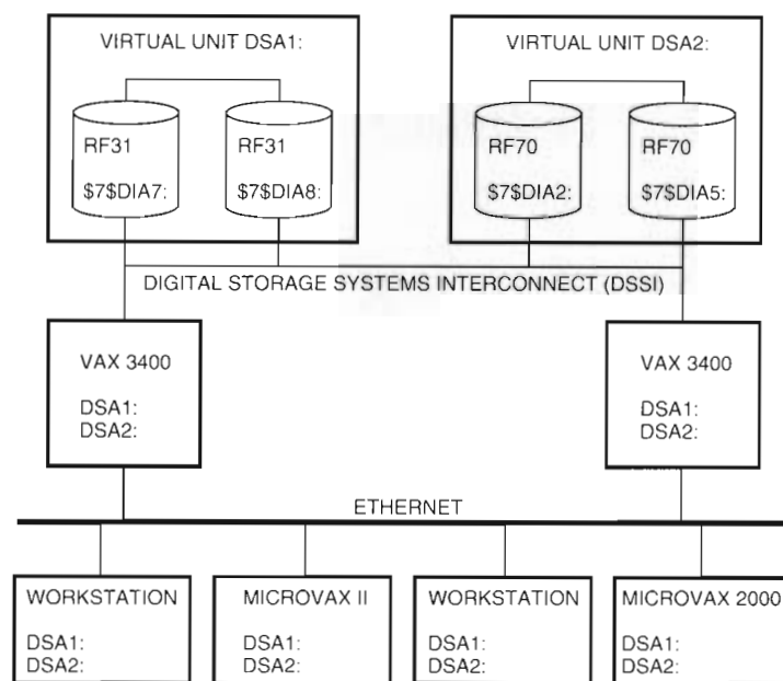
Figure 1 Phase II Shadow Set for a Dual-host DSSI Configuration
