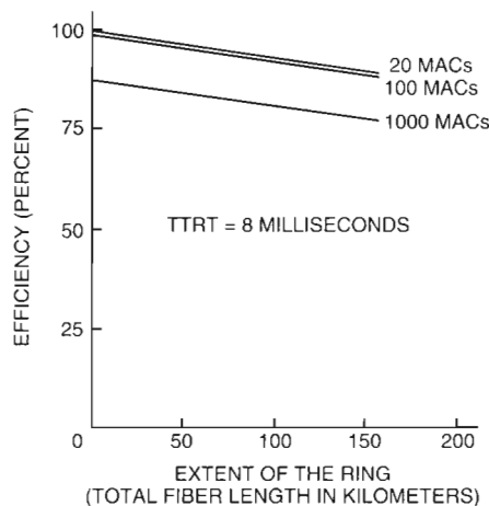
Figure 6 Efficiency as a Function of the Extent of the Ring
