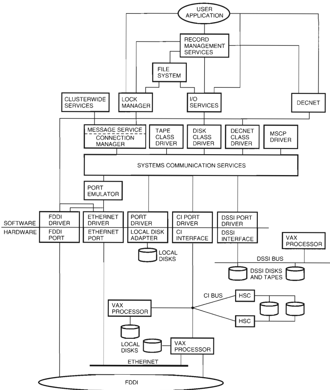
Figure 1 VAXcluster System Architecture
