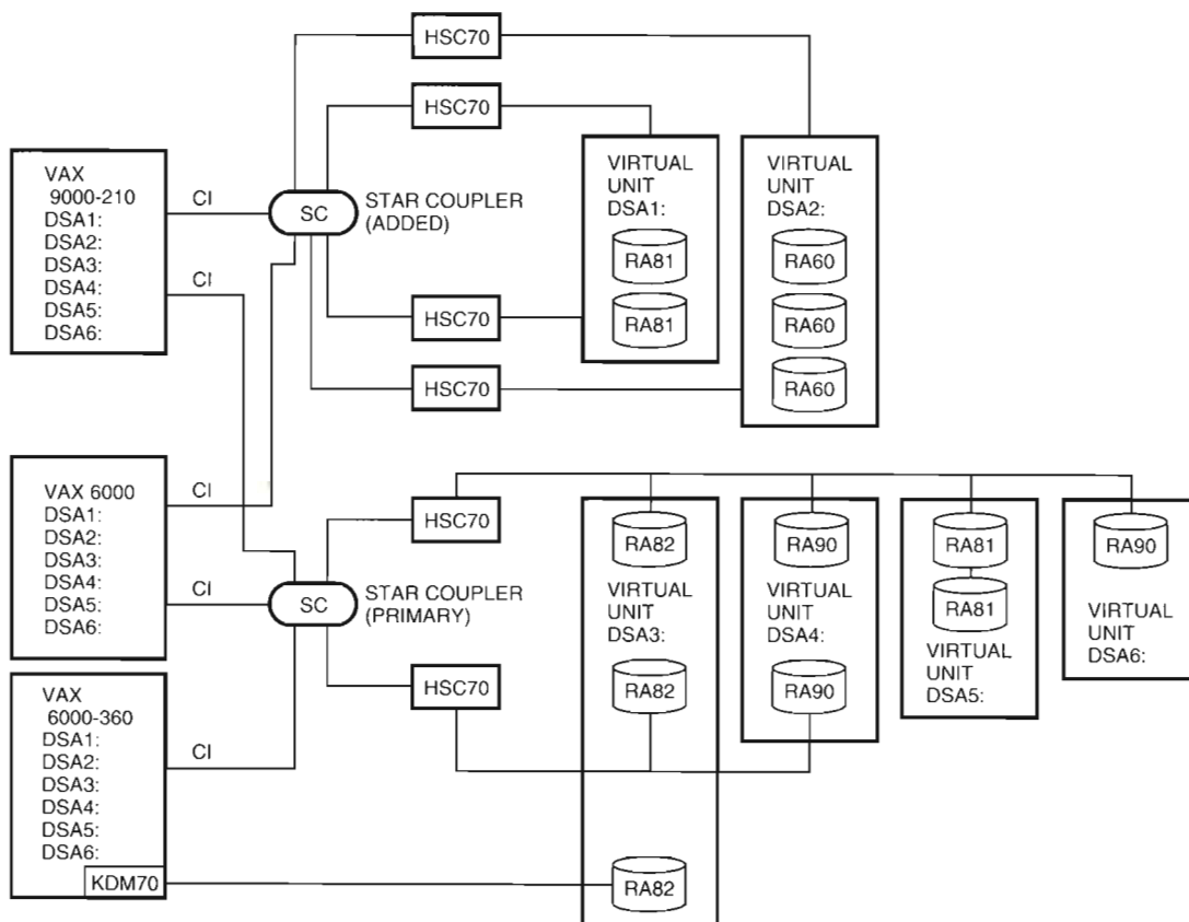
Figure 2 Clusterwide Shadow Sets for an HSC Configuration with Multiple CI Buses
