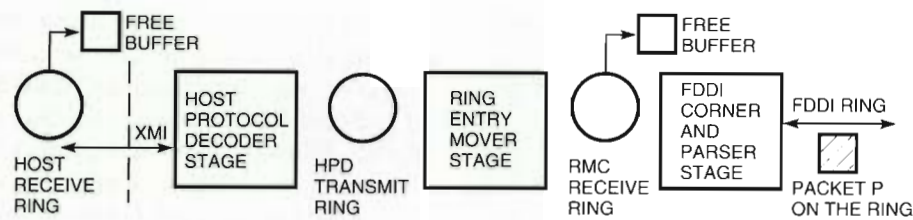
(a) Receive Stream - Packet on the FDDI Ring
