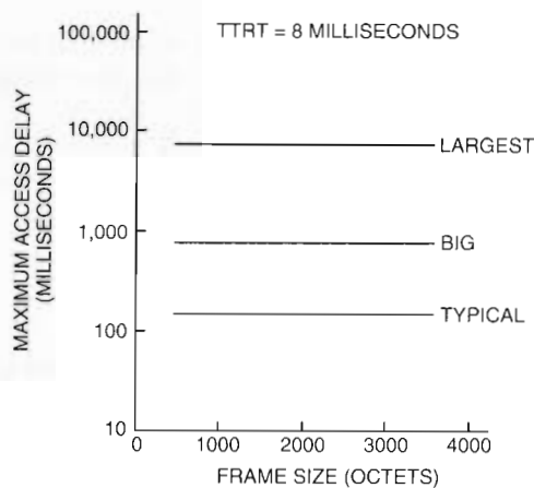
Figure 11 Maximum Access Delay as a Function of the Frame Size
