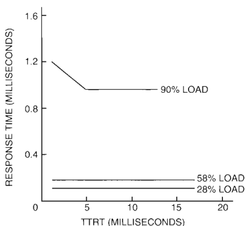
Figure 5 Response Time as a Function of TTRT
