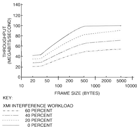
Figure 8 Transmit Throughput as a Function of the Frame Size for the XMI (I/O) Bus Configuration
