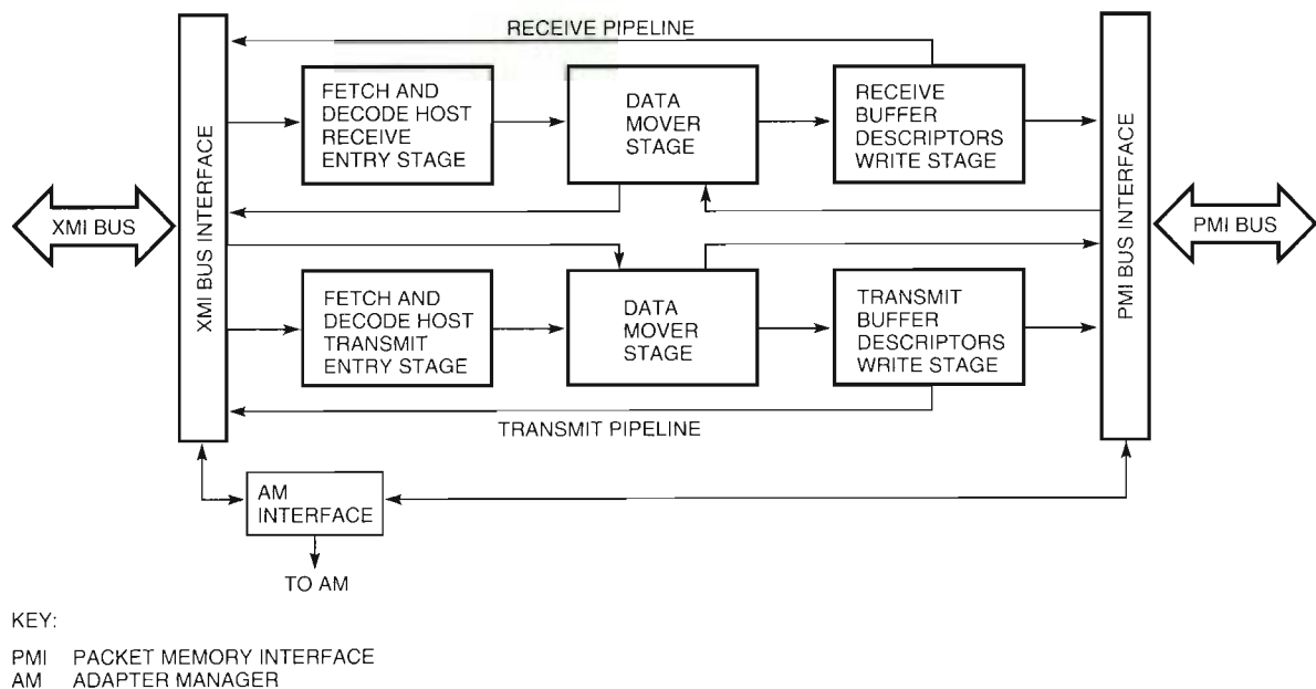
Figure 7 Host Protocol Decoder Stage
