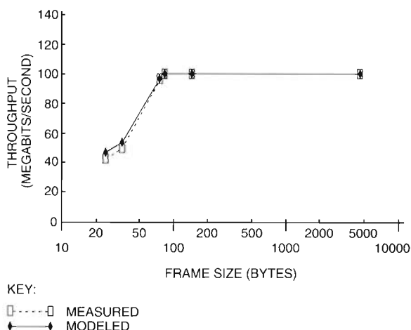
Figure 13 Validation of Receive Throughput Results
