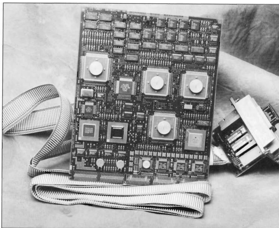
Figure 9 The DEMFA Board
