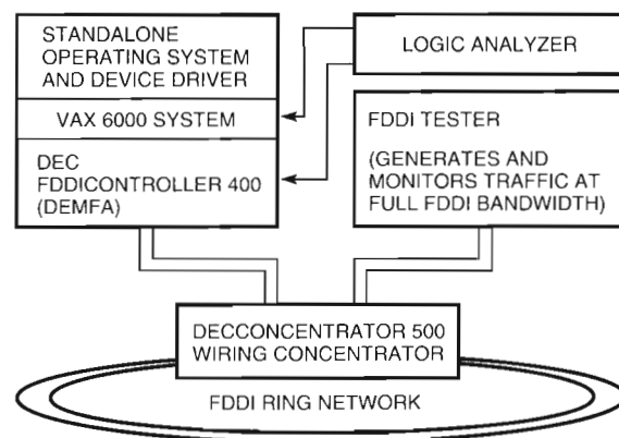
Figure 12 Laboratory Setup for DEMFA Performance Measurements
