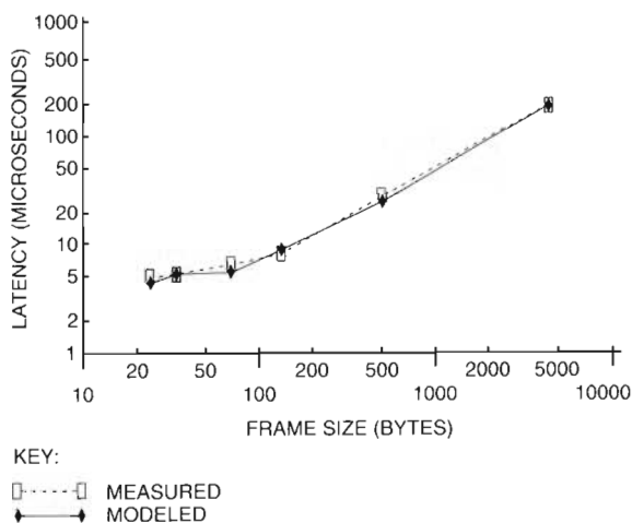
Figure 14 Validation of Receive Frame Latency Results
