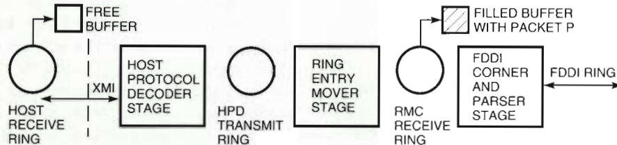
(b) Receive Stream - Packet at the RMC Receive Ring
