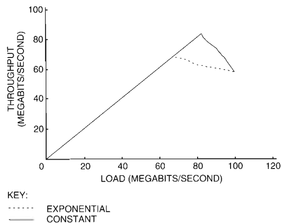
Figure 3 Receive Throughput as a Function of the Load for a 33-byte Frame
