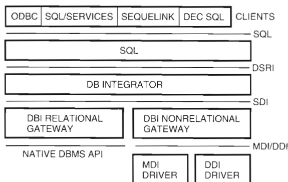
Figure 5 DB Integrator Architecture
