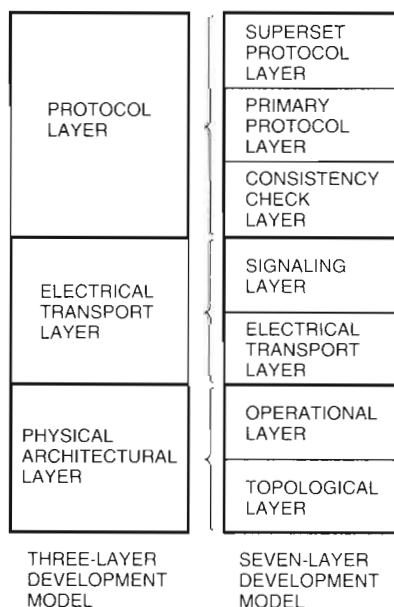
Figure 1 Comparison of Conventional Three-layer Model with Seven-layer Platform Development Model
