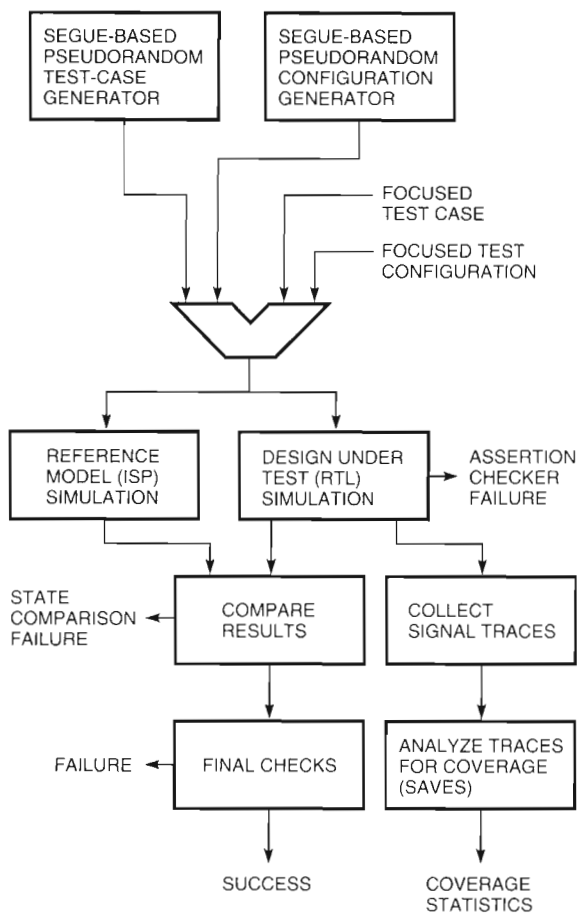
Figure 1 Design Verification Test Environment
