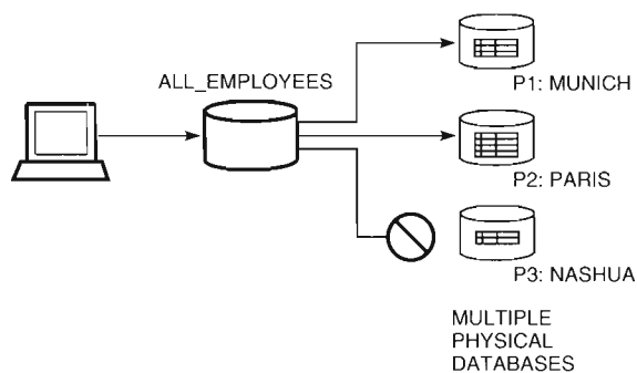
Figure 11 High Availability with Partitioned Views
