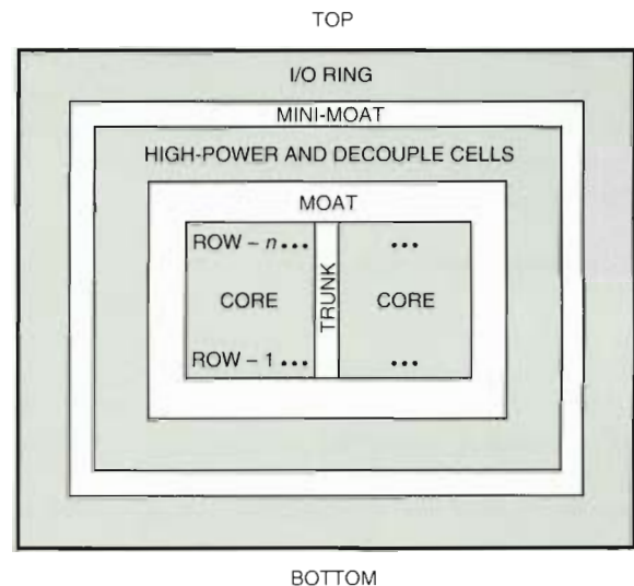
Figure 2 CSALT Die Architecture
