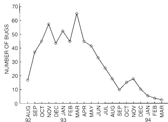
Figure 2 Bug Rate as a Function of Time
