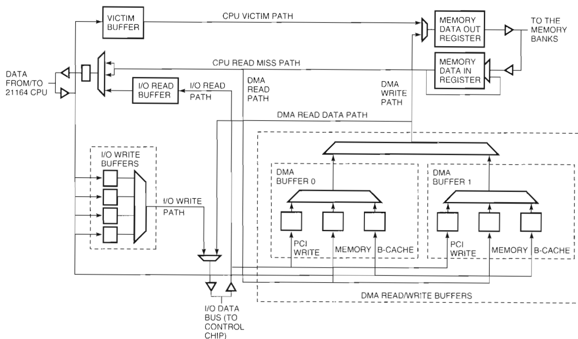
Figure 2 Data Slice Block Diagram
