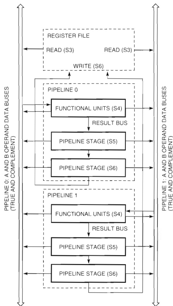
Figure 8 E-box Pipeline
