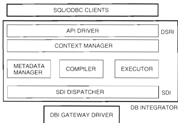
Figure 6 DB Integrator Components
