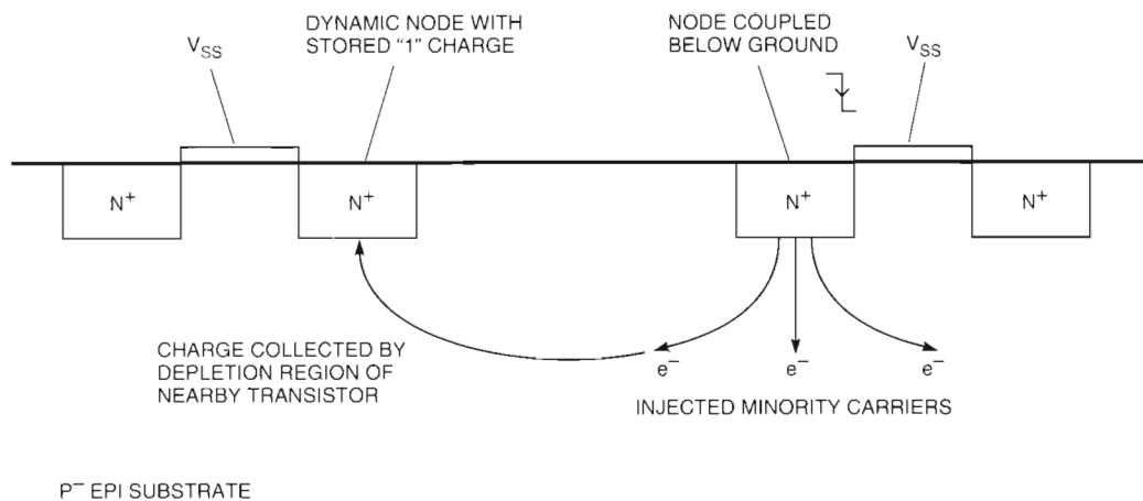
Figure 12 Dynamic Node Corruption Caused by Minority Carrier Injection
