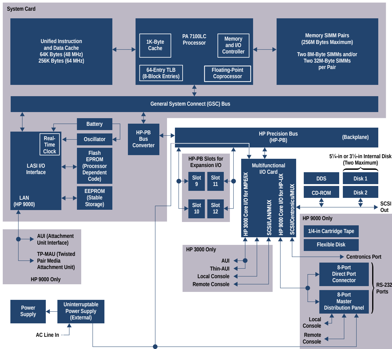
Fig. 1. Block diagram for the HP 9000 Series 800 Models Ex5 and the HP 3000 Series 9x8 business servers.
