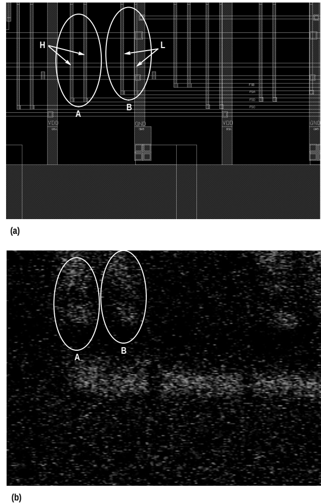
Fig. 8. (a) FS[ABCD] bus artwork. (b) Voltage contrast image of FS[ABCD] bus in metal 1 showing correct firing of the lines in circle A and the incorrect firing of lines in circle B.
