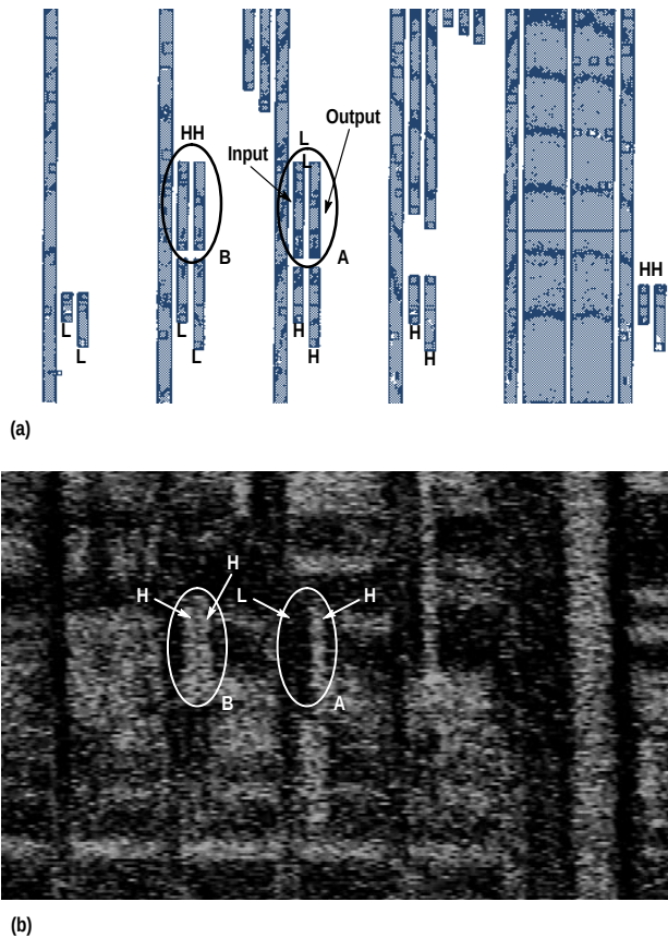
Fig. 7. (a) Metal 3 plot of Zero_topH buffer with failing input/output pair A. (b) Voltage contrast image of victimized buffer with failing input/output pair A.
