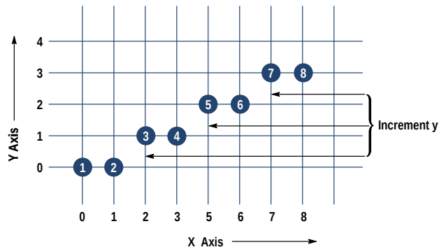
Fig. 8. Pixel representation of a vector that starts at coordinate 0,0, is 8 pixels long, and has a slope of 1/2.
