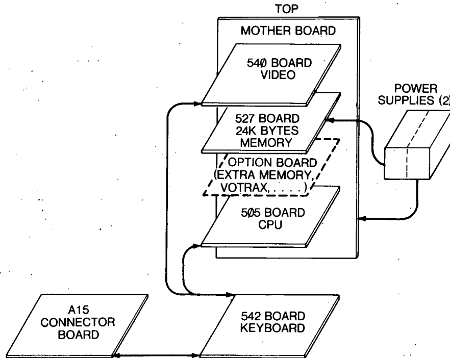
Fig. 23 Board Layout
