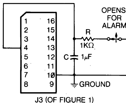
Fig. 21 Temperature Alarm
