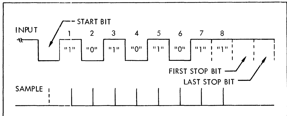
Figure 4-5. Input Character Sampling
