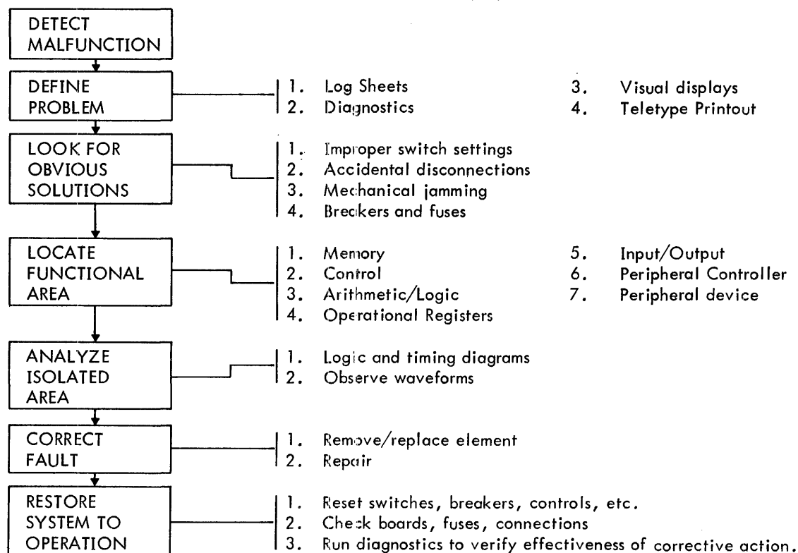
Figure 2-16. General Troubleshooting Steps
