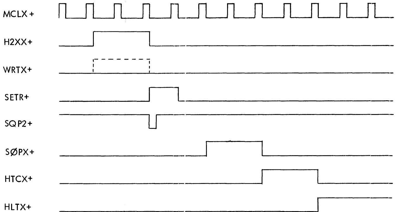
A. TIMING FOR STORE AND INCREMENT
