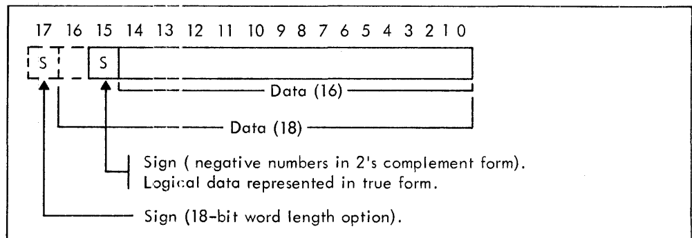
Figure 2-4. Data Word Format
