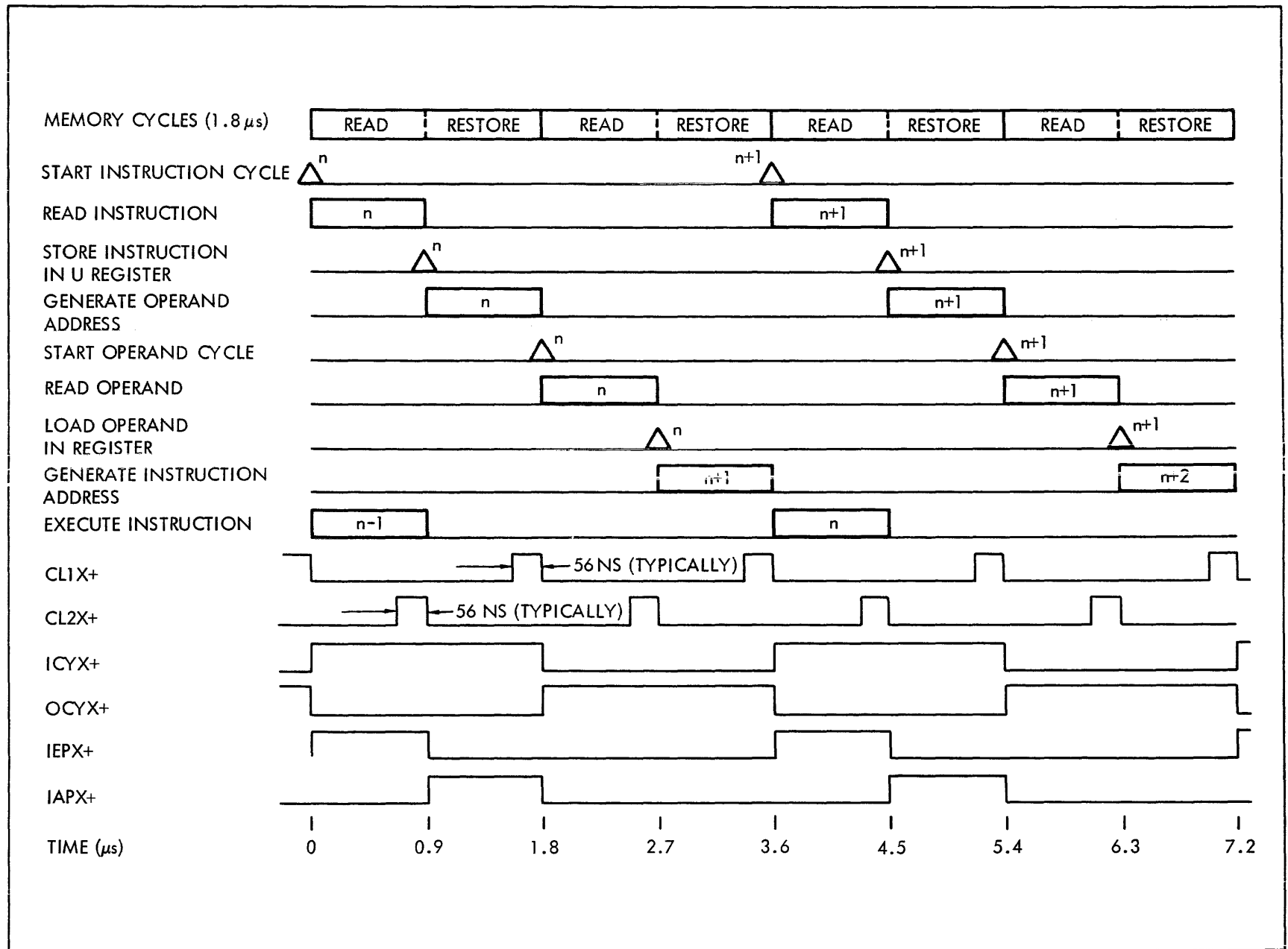
Figure 2-13. Sequence for Operand Access from Memory
