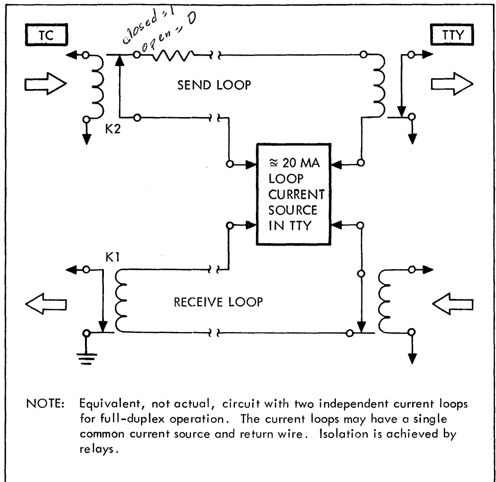
Figure 4-3. Typical Full-Duplex Teletype-TC Connection for Model 33-ASR in Factory-Modified System
