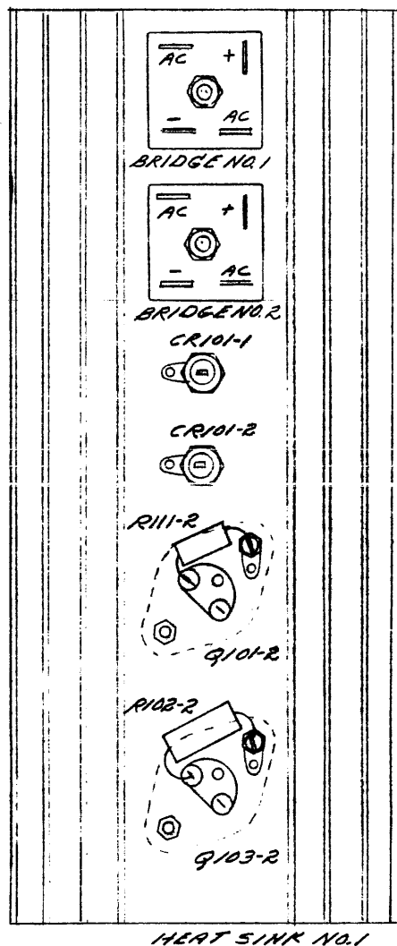
HEAT SINK NO. 1
