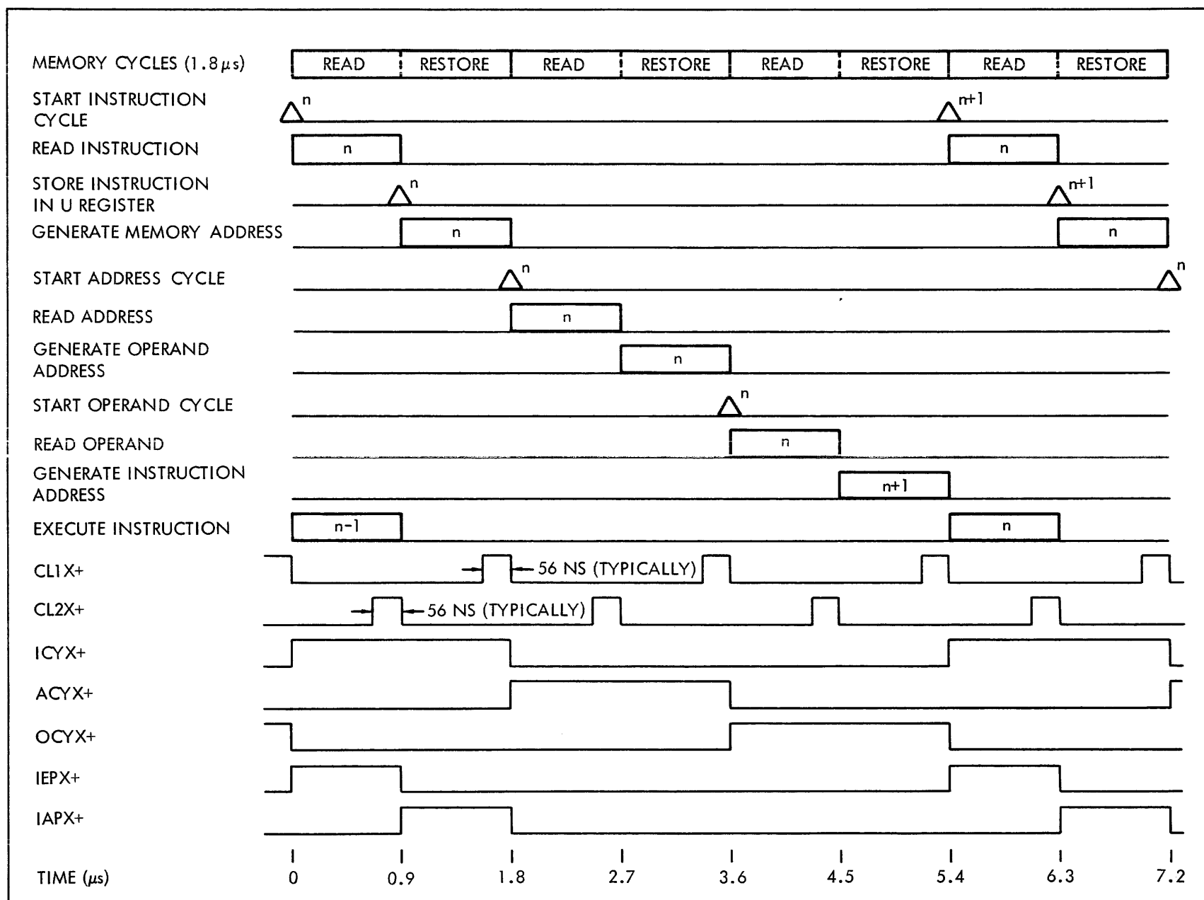
Figure 2-15. Sequence for Indirect Operand Access
