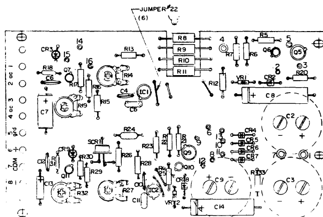
PC BOARD ASSY #522251
