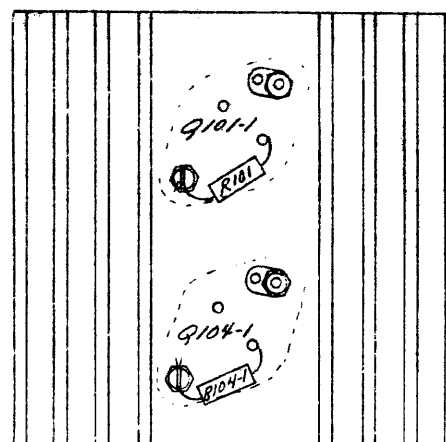
VIEW B-B
