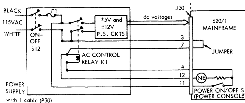
Diagram A. Mainframe Connections.
