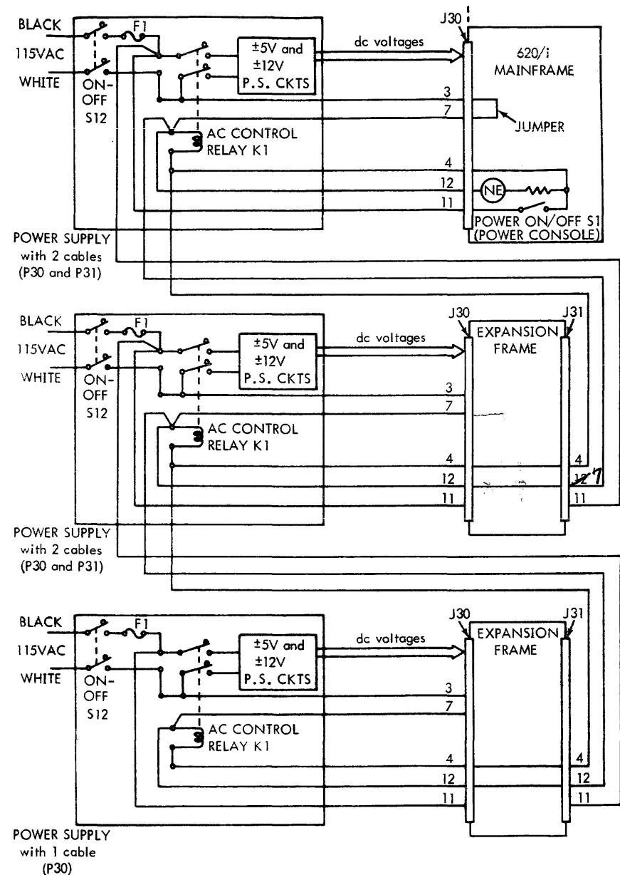
Diagram B. Mainframe Plus Two Expansion Frames Connections.
