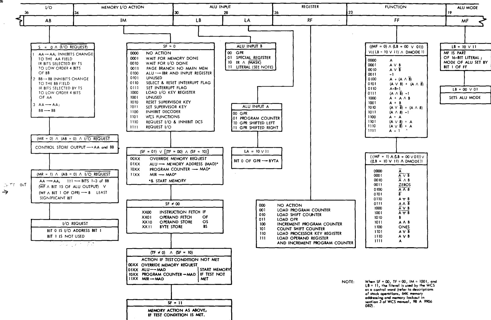
Figure 2-1. Microinstruction Fields (2 of 3)
