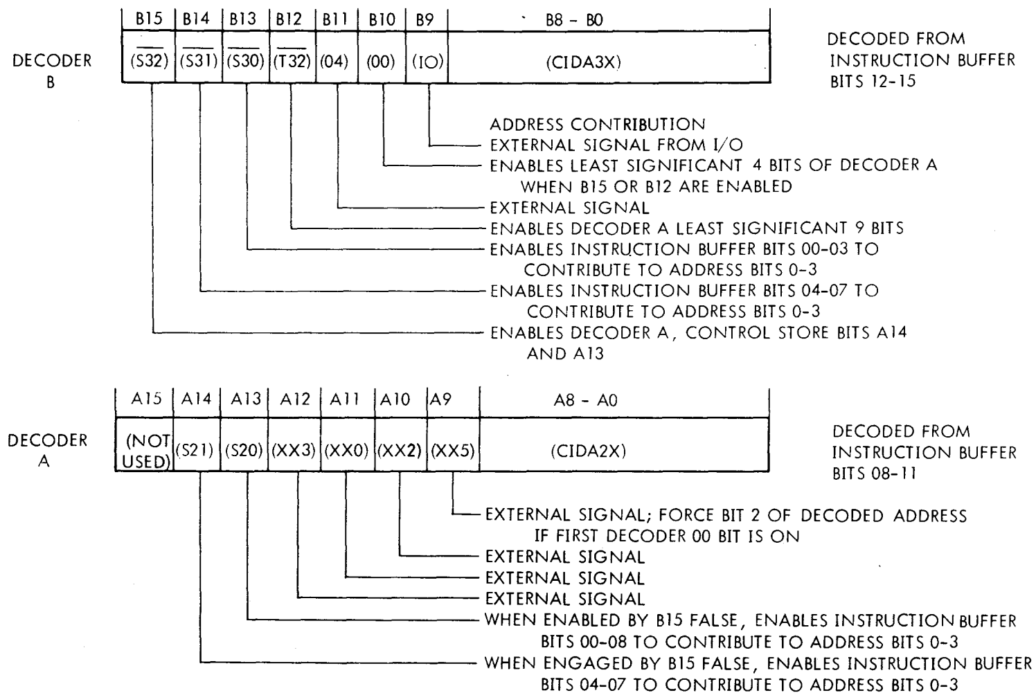
Figure 8-1. Decoder Control Store Format
