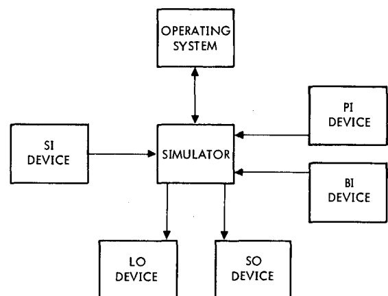
Figure 6-2. Microsimulator Data Flow
