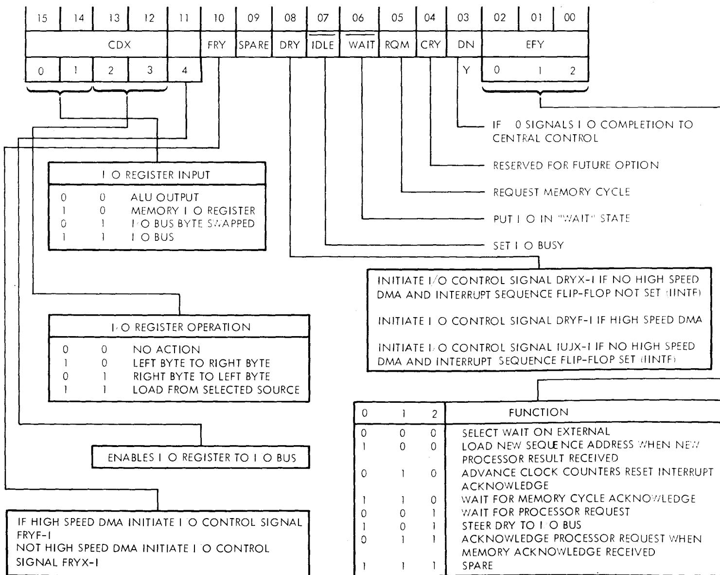
Figure 8-3. I/O Microinstruction Format
