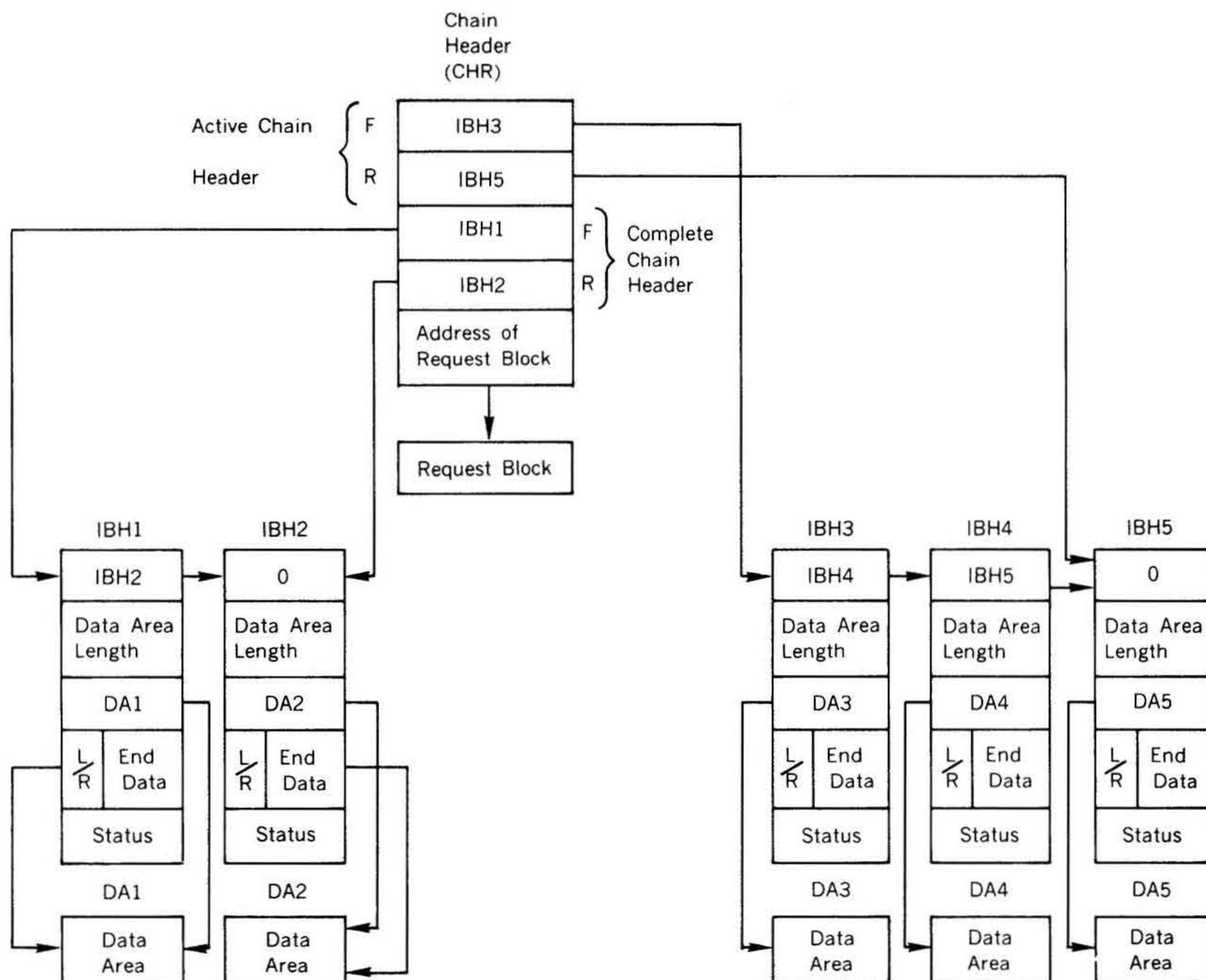
Figure 7-4. Relationship of CHR and IBHs
