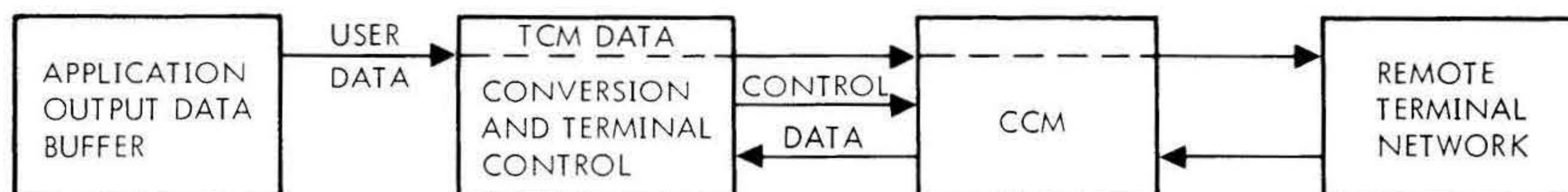
Figure 1-2. Data Flow From Application To Terminal
