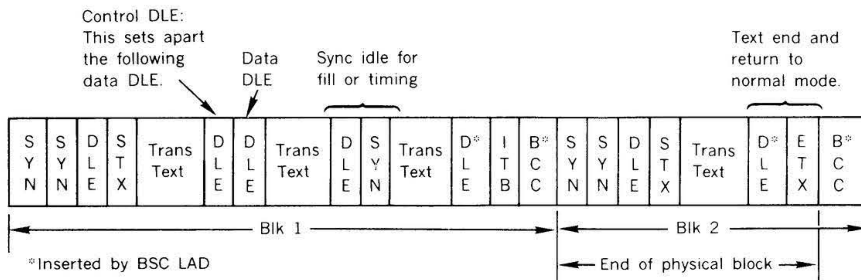
Figure 8-4. Transparent Data Block
