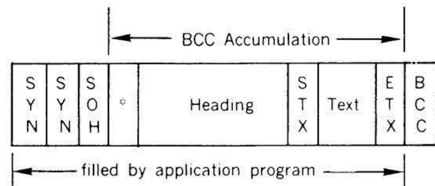
Figure 8-1. Regular Message Format
