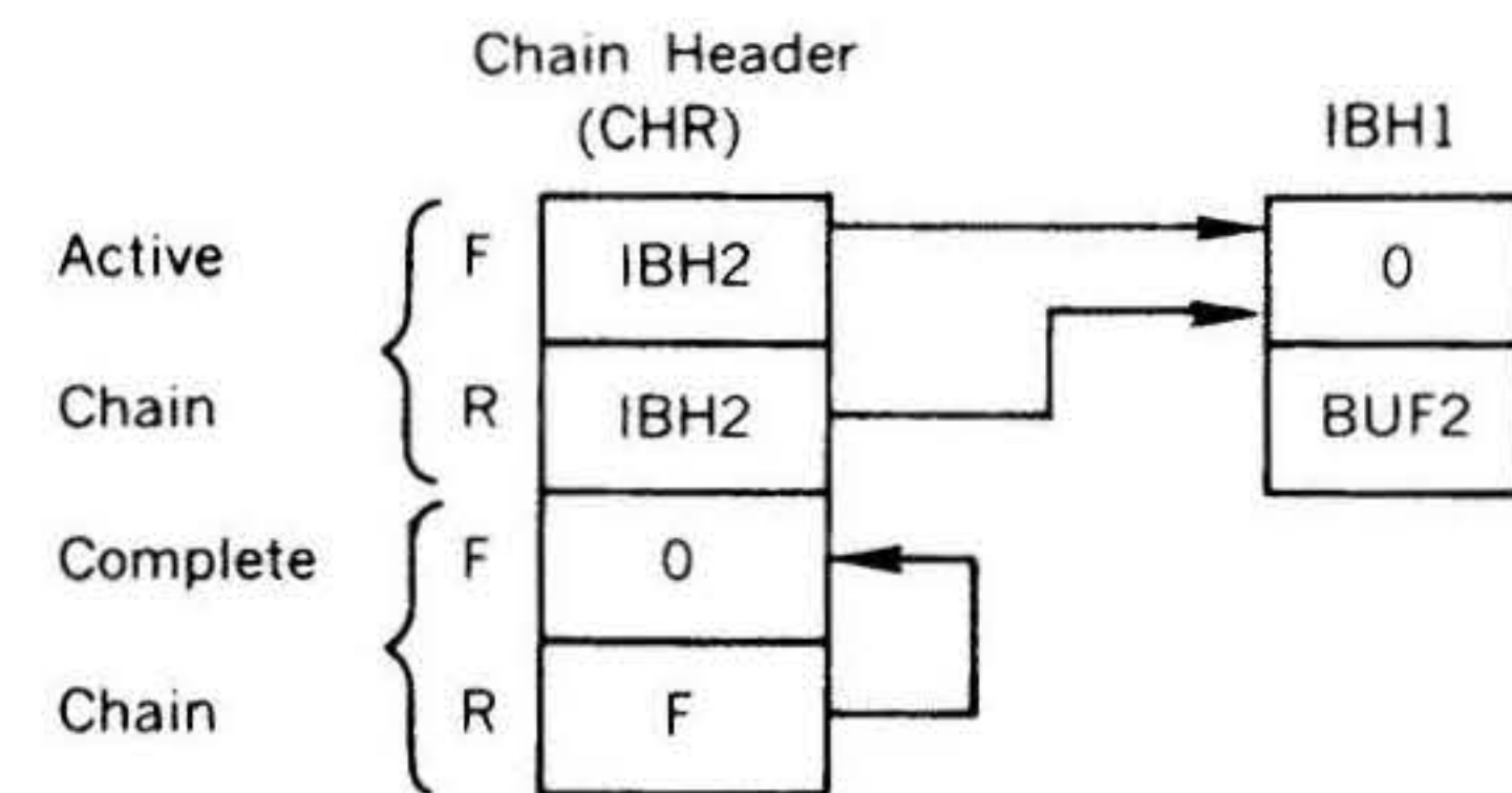
Figure 7-3. Contents of CHR and IBHs Before and After GETQ
