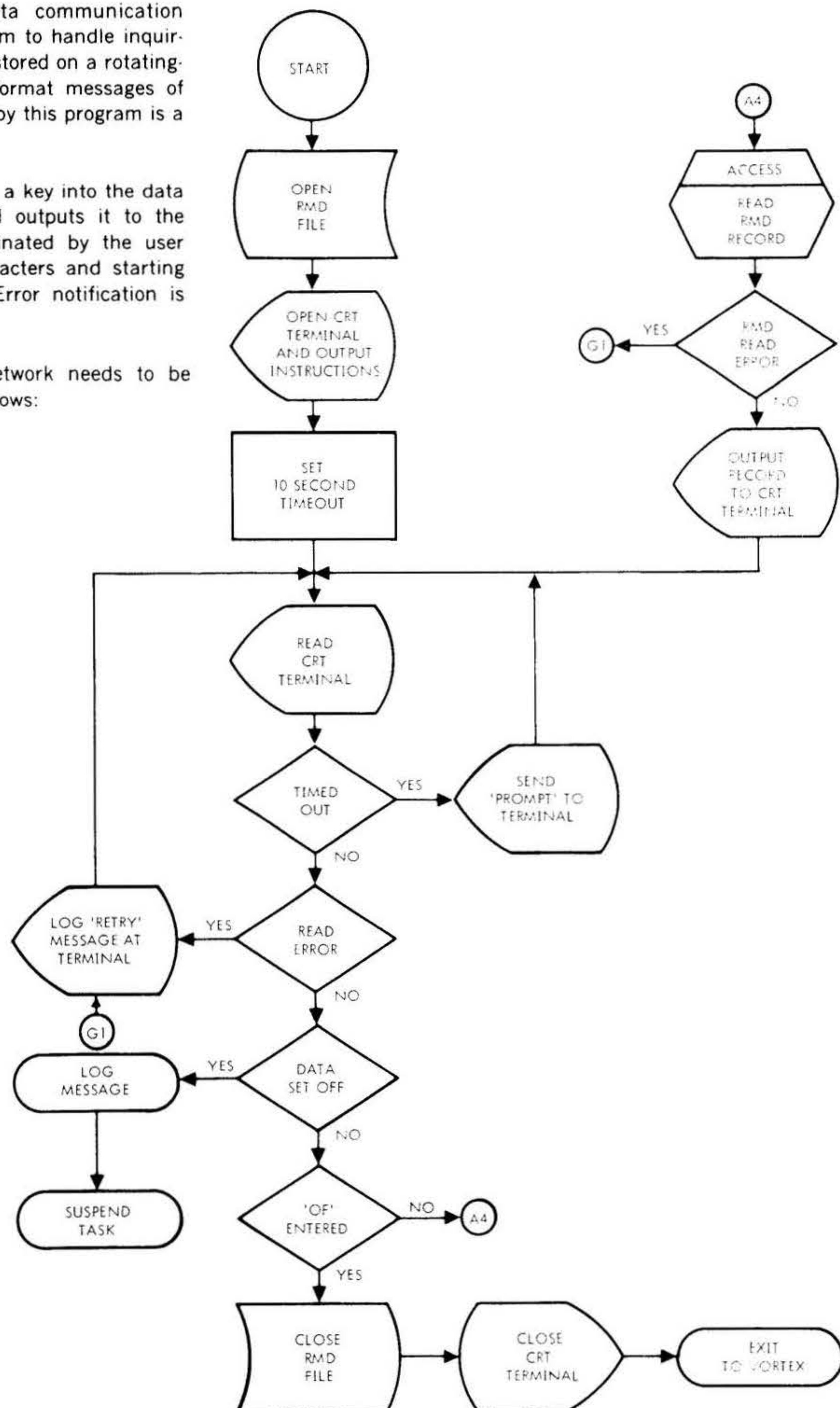
Figure 12-1. Flowchart of VTAM Application
