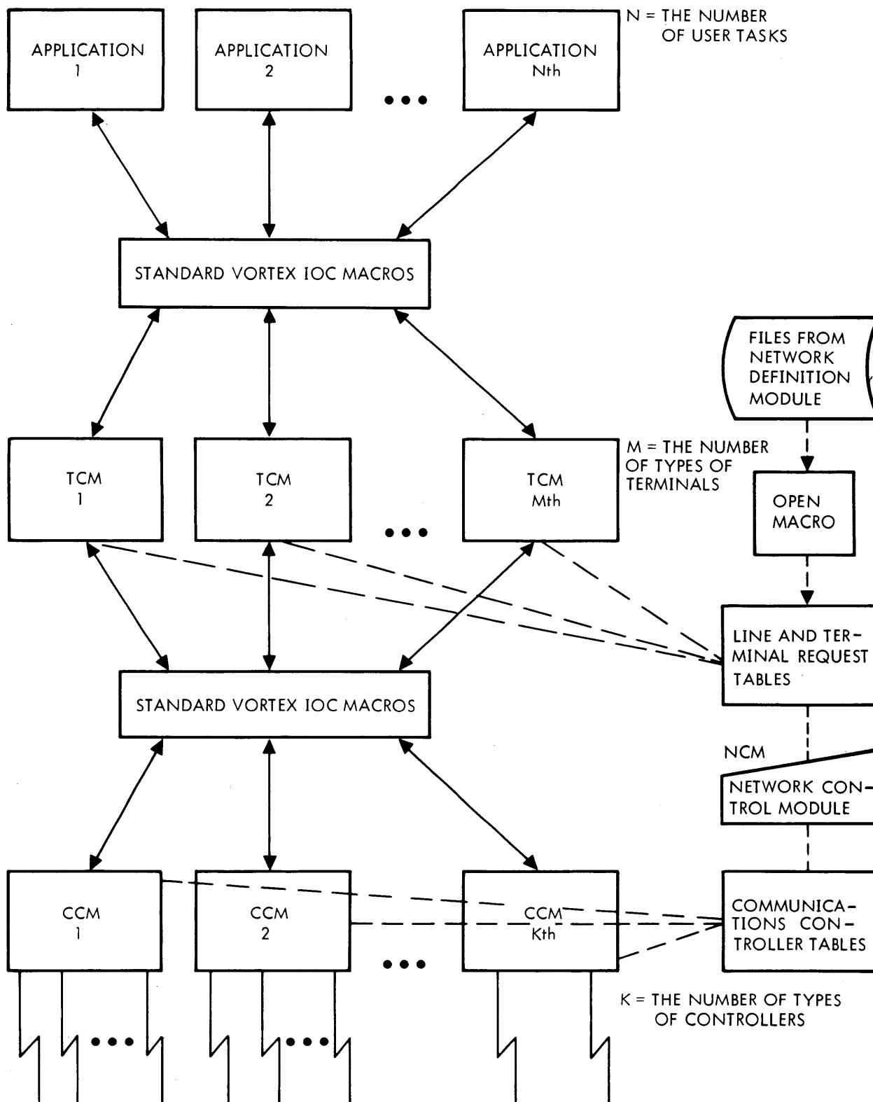
Figure 1-1. Structure of VTAM
