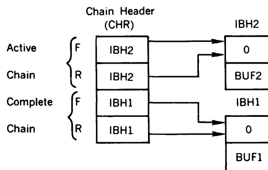
Figure 7-2. Contents of CHR and IBHs During READ
