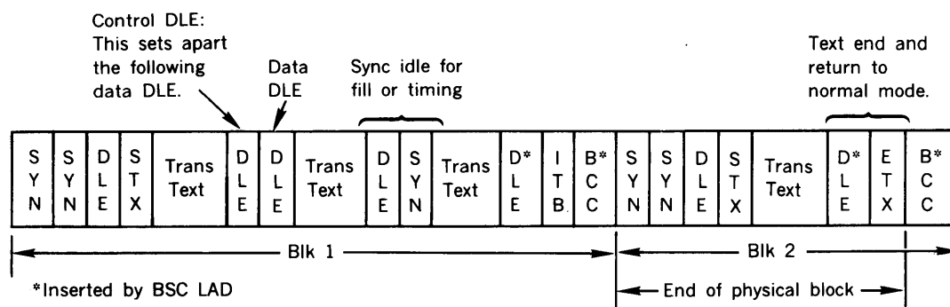
Figure 8-4. Transparent Data Block
