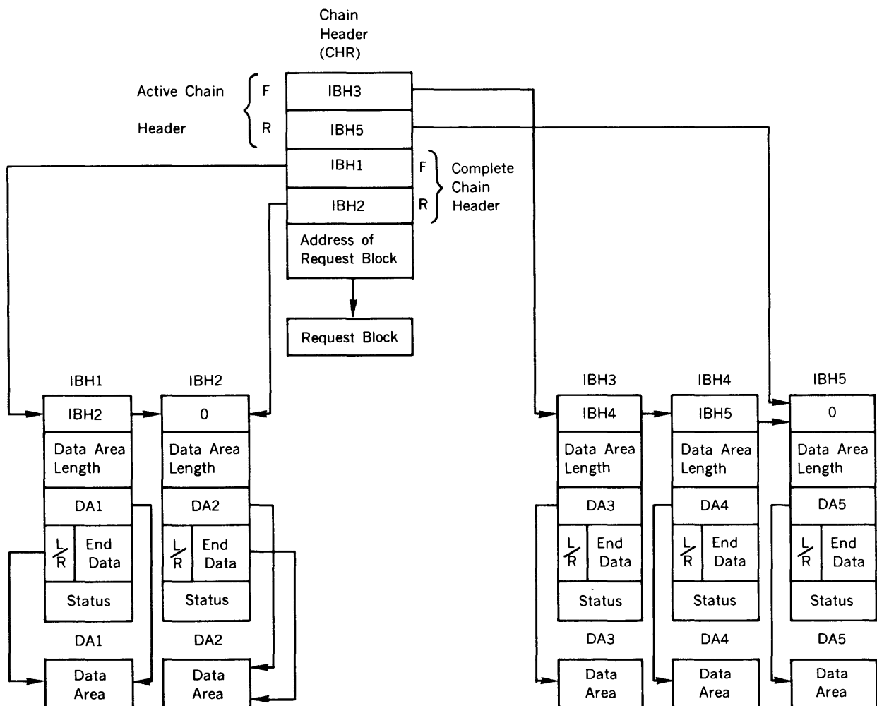
Figure 7-4. Relationship of CHR and IBHs
