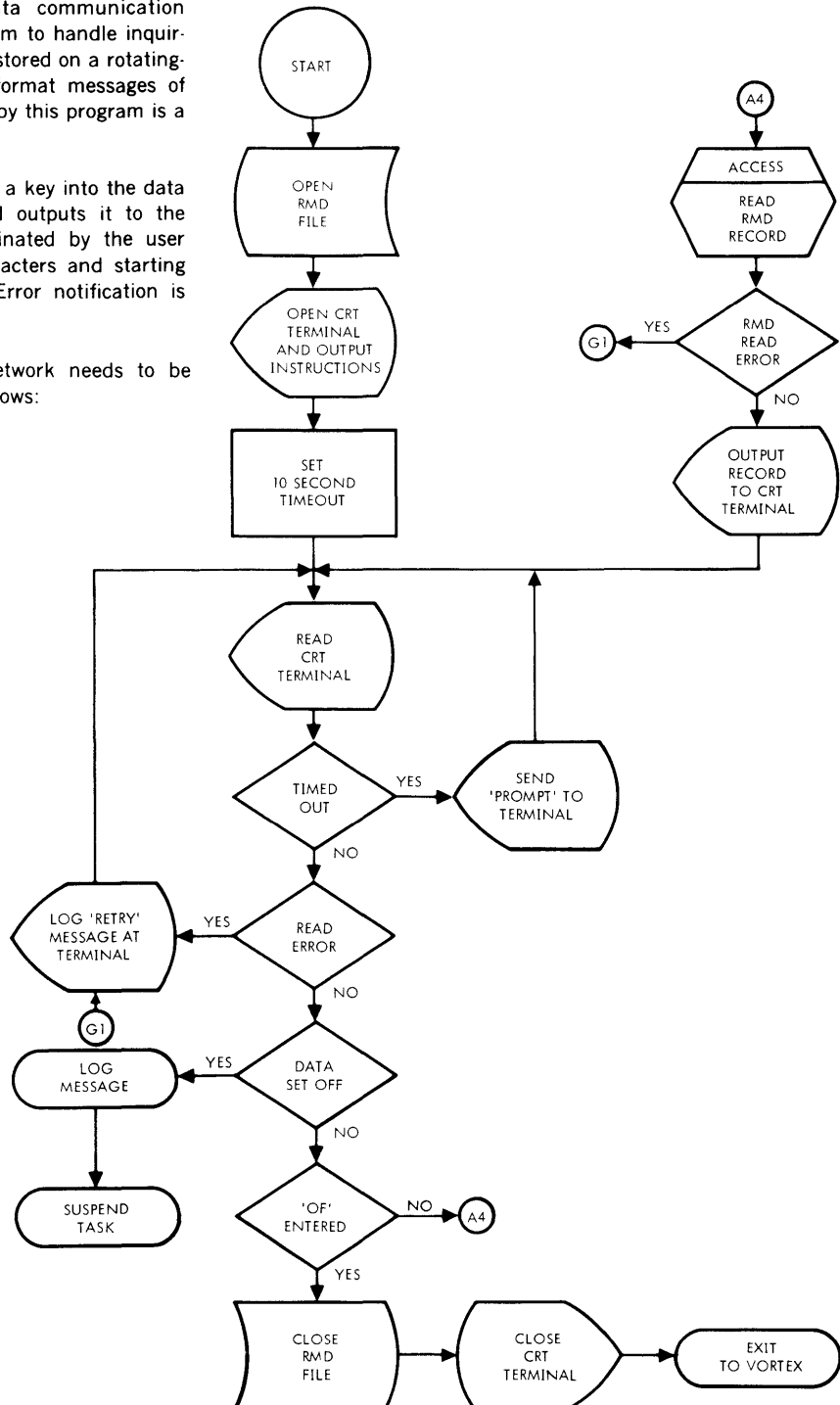
Figure 12-1. Flowchart of VTAM Application
