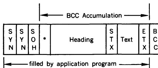
Figure 8-1. Regular Message Format
