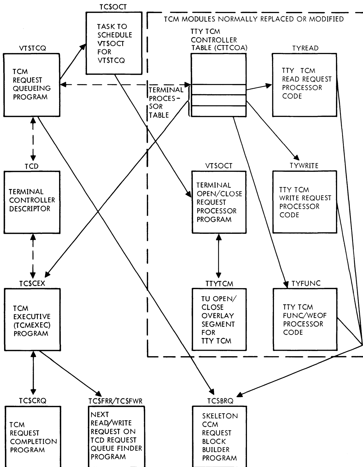
Figure 10-1. VTAM TCM and TTY TCM Modules
