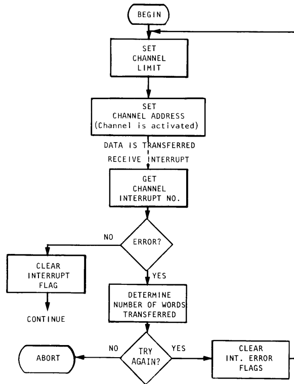
Figure 2-7. Basic I/O program flowchart
