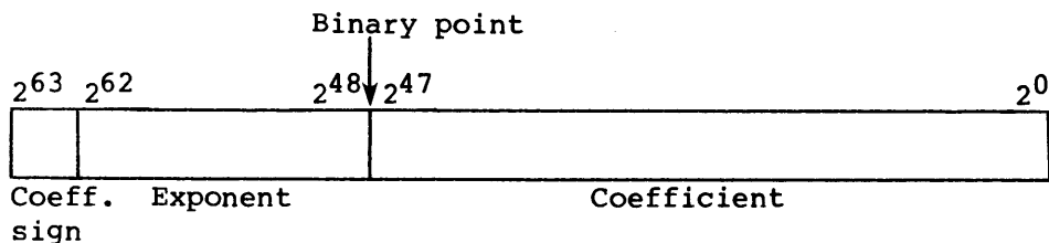
Figure 4-5. Floating-point data format
