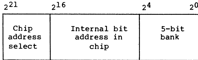
Figure 2-2. Memory address (32 banks)
