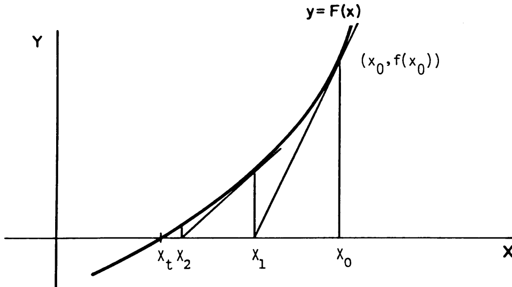
Figure 4-9. Newton's method
