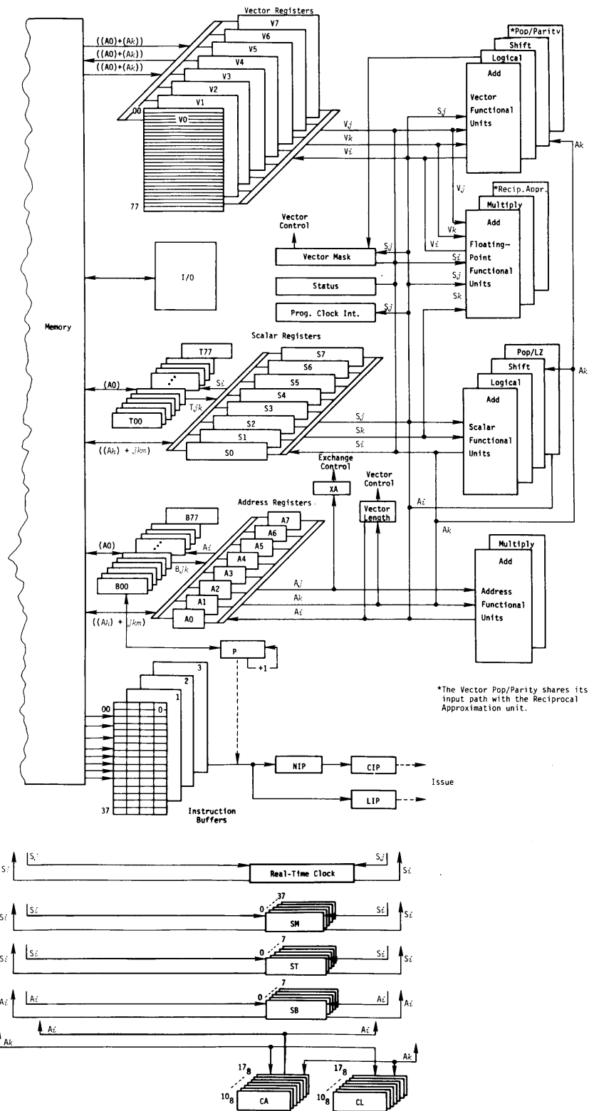
Figure 1-3. Control and data paths for a CPU
