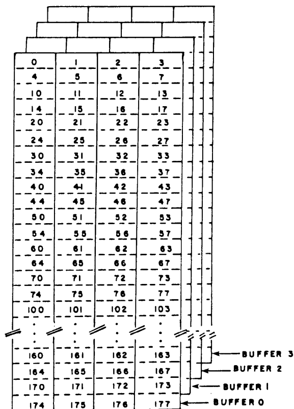
Figure 3-2. Instruction buffers
