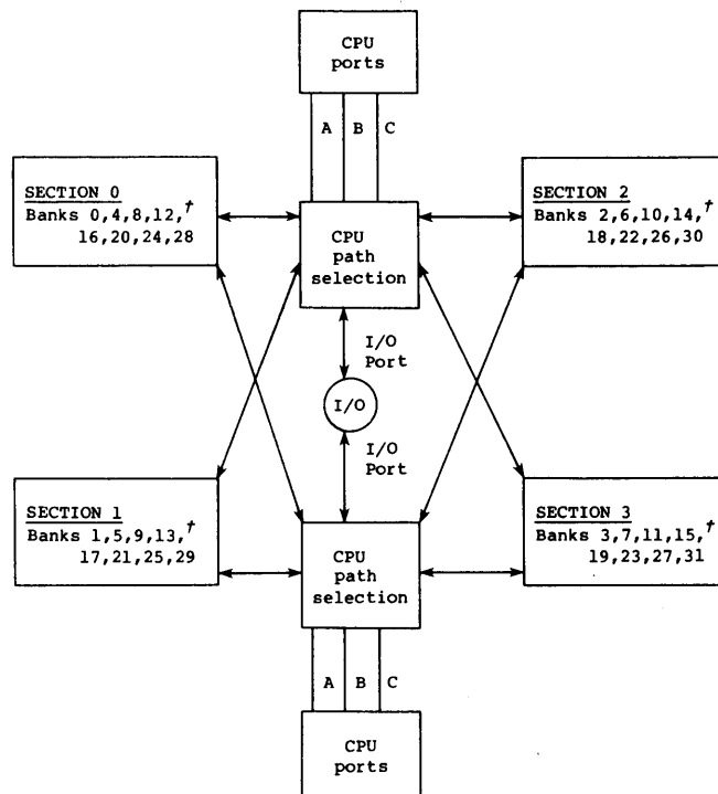
Figure 2-1. Central Memory organization
