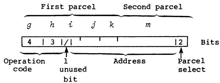
Figure 5-5. 2-parcel instruction format with combined i , j , k , and m fields
