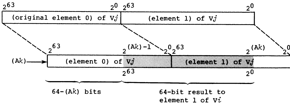
Figure 5-10. Vector right double shift, second element, VL greater than 1
