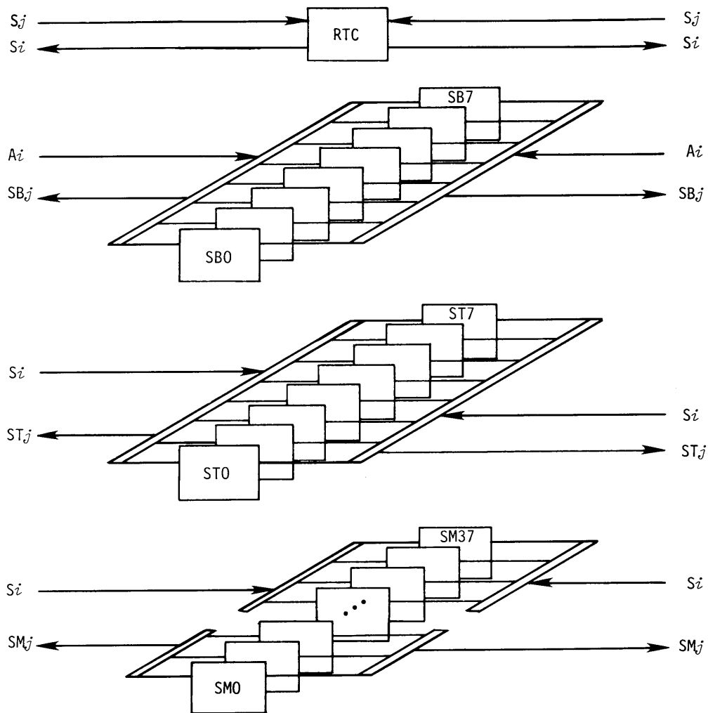
Figure 2-6. Shared registers
