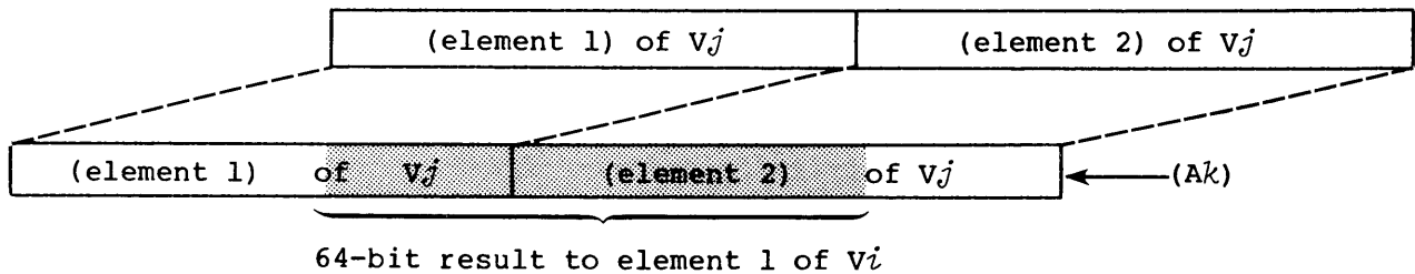
Figure 5-7. Vector left double shift, second element, VL greater than 2
