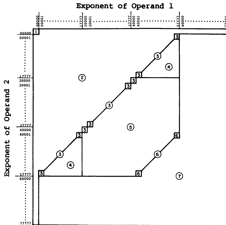
Figure 4-6. Exponent matrix for Floating-point Multiply unit
