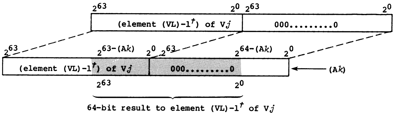
Figure 5-8. Vector left double shift, last element
