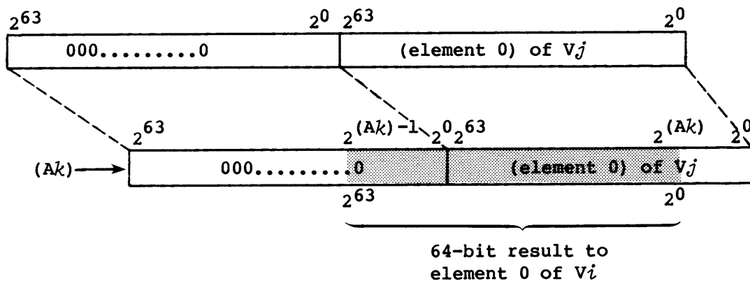
Figure 5-9. Vector right double shift, first element
