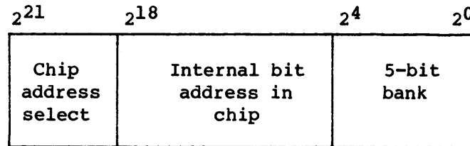
Figure 2-2. 32-bank memory address
