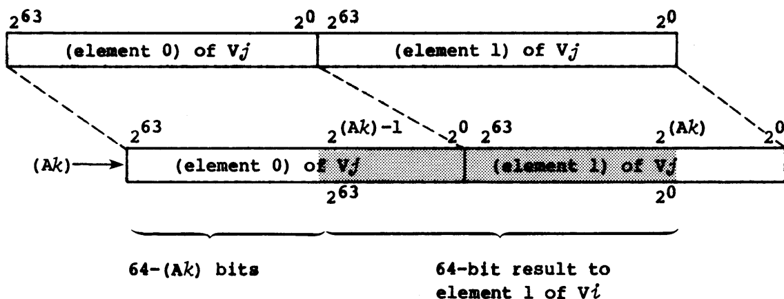
Figure 5-10. Vector right double shift, second element, VL greater than 1
