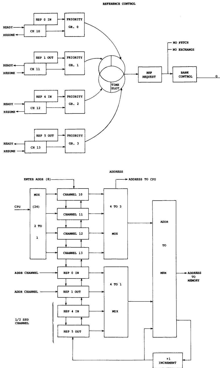
Figure 2-8. Channel I/O control
