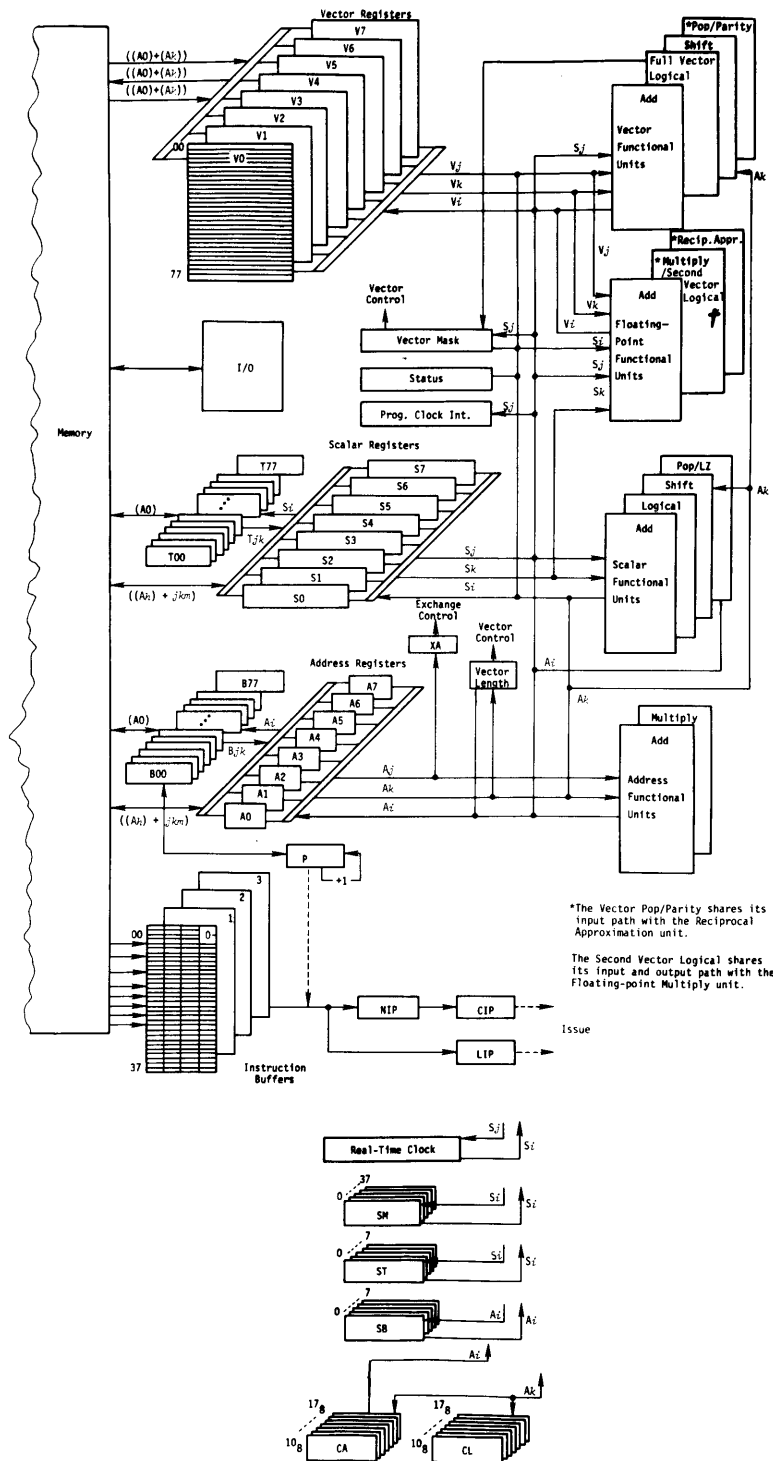
Figure 1-3. Control and data paths for the CPU
