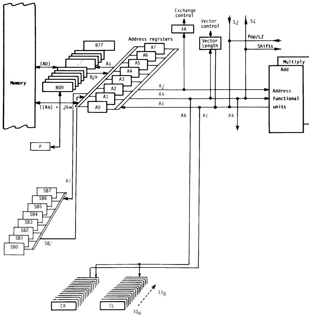
Figure 4-1. Address registers and functional units
