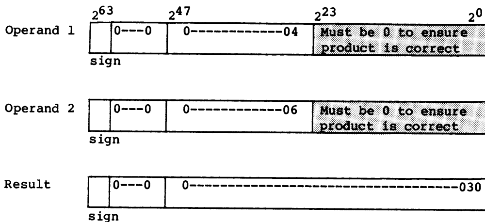
Figure 4-7. Integer multiply in Floating-point Multiply functional unit
