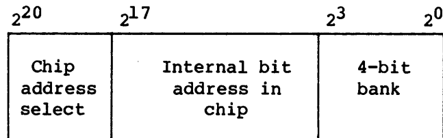
Figure 2-3. 16-bank memory address
