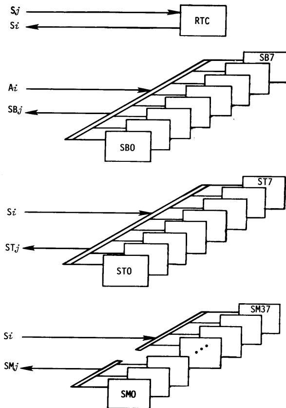
Figure 2-6. Shared registers and real-time clock
