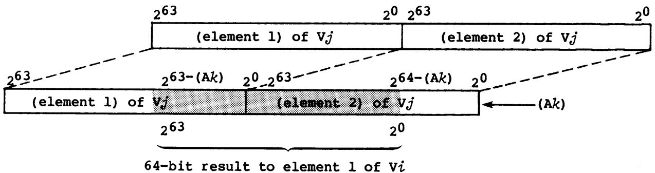
Figure 5-7. Vector left double shift, second element, VL greater than 2
