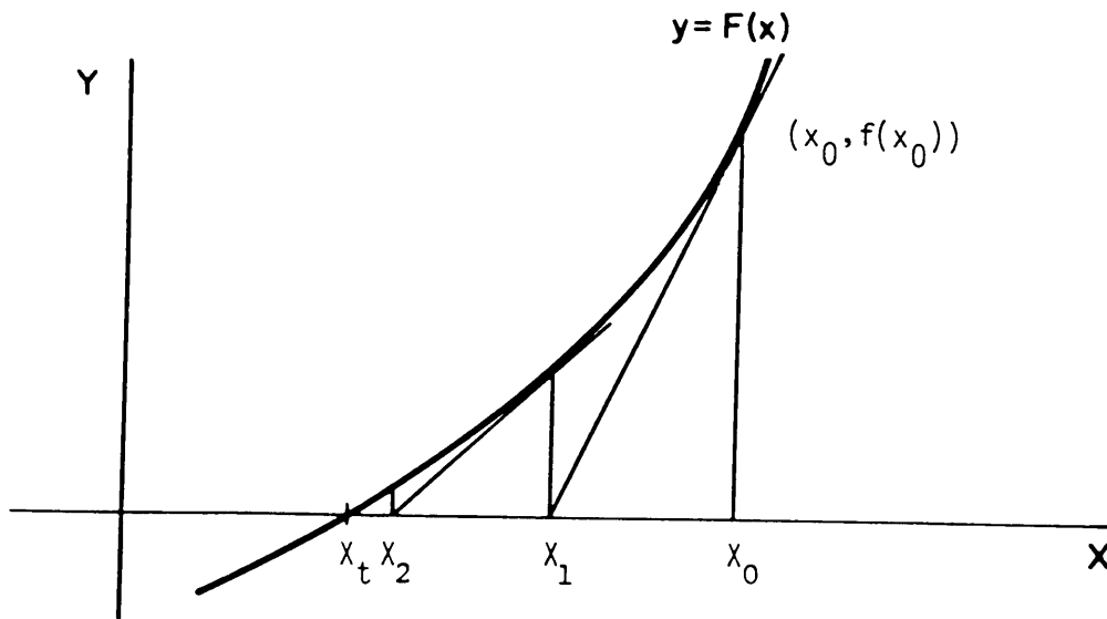
Figure 4-10. Newton's method
