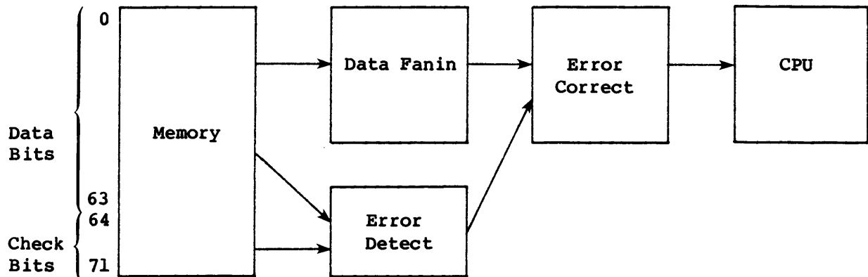
Figure 2-4. Memory data path with SECDED
