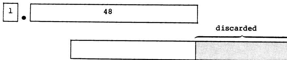
Figure 4-8. 49-bit floating-point addition
