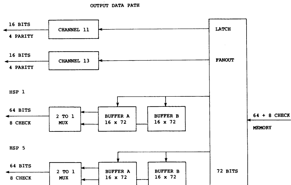
Figure 2-9. Input/output data paths
