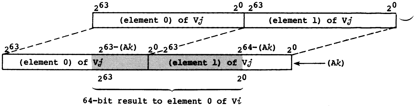
Figure 5-6. Vector left double shift, first element, VL greater than 1
