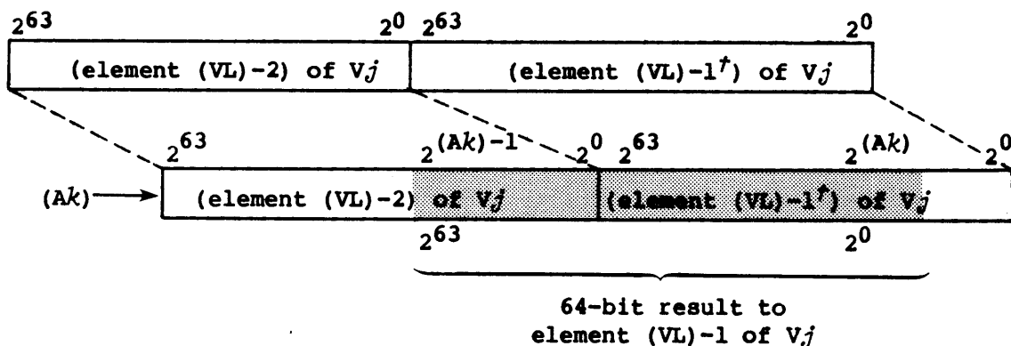
Figure 5-11. Vector right double shift, last operation
